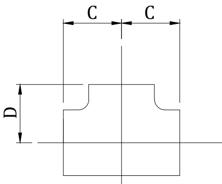
EQUAL TEES
